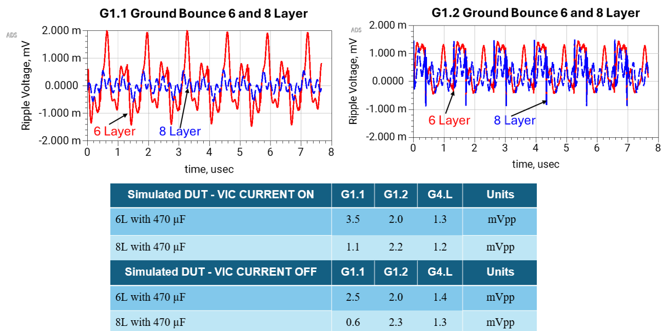
Figure 22 - Simulated Ground Bounce at Locations G1.1 and G1.2
