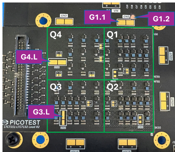
Figure 11 - Ground Bounce Measurement Test Points on DUT
