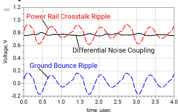
6 Layer PCB – Total Differential Noise 49mV
