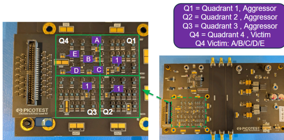
Figure 18 - Crosstalk Measurement Test Points on DUT
