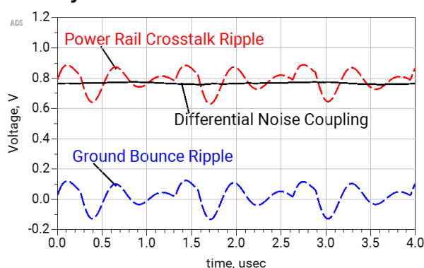
8 Layer PCB – Total Differential Noise 3mV
